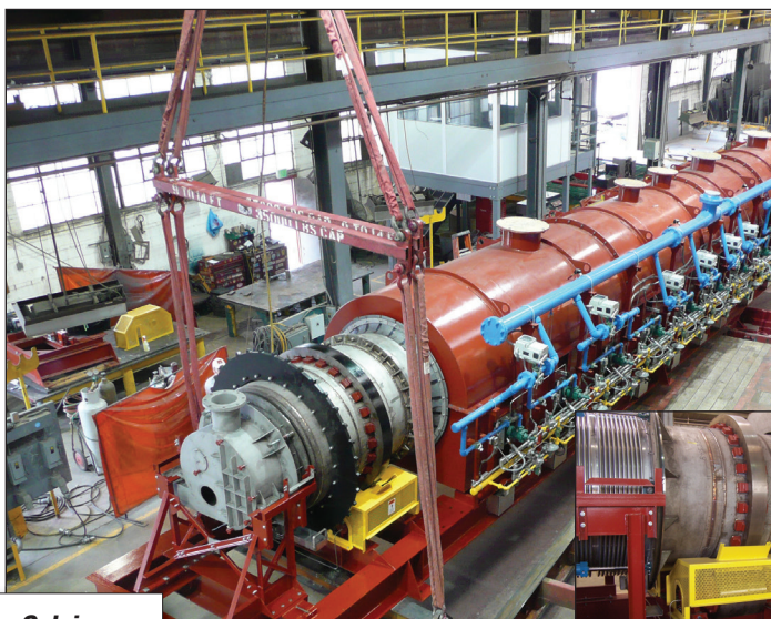
Calciners
